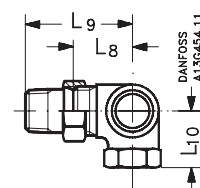
Winkeleck
