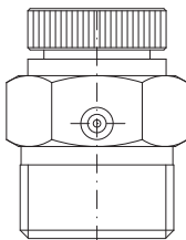
Automatic air bleeder valve G 1/8", 1/4", 3/8"
