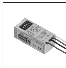
ELS-ZNE Electronic overrun timer with variable adjustable overrun times Assembly: flush-mounted box behind switch
