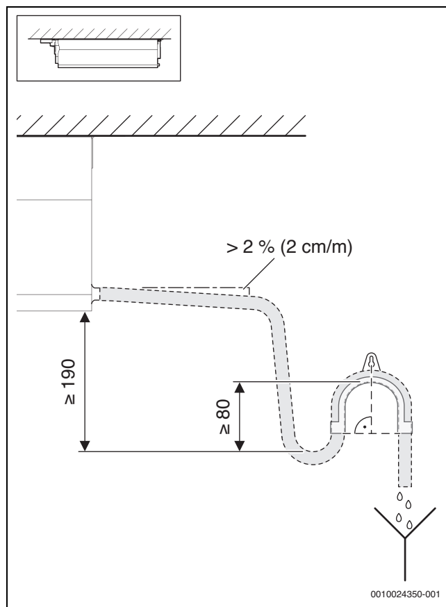
4 CKS 100
