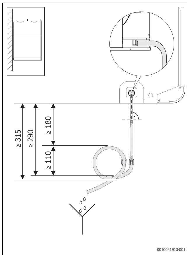
6 HRV-CKS
