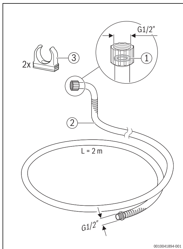
2 HRV-CKS
