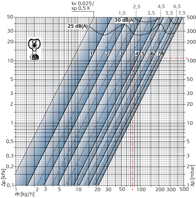
Regeldifferenz [xp] 2,0 K
